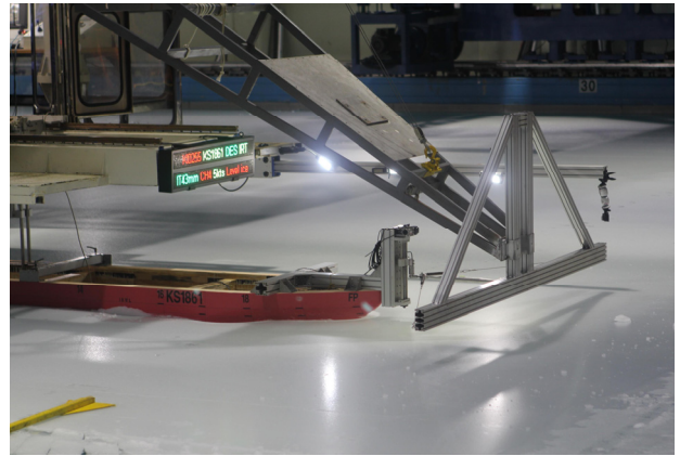
Fig. 5 Bow towing test in level ice
