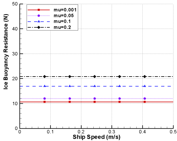
Fig. 11 Ice buoyancy resistance with an ice sheet of 42.5 mm thickness
