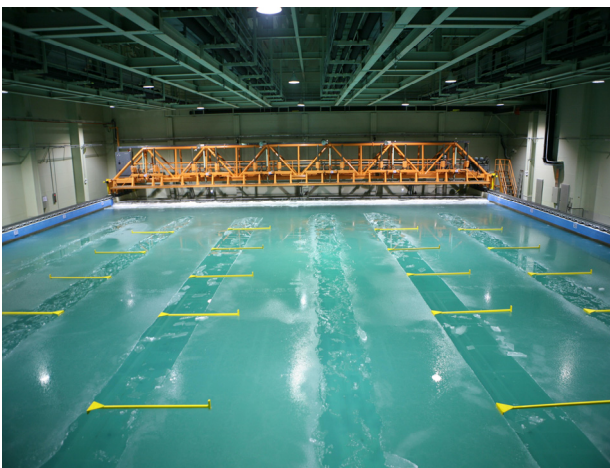
Fig. 3 Photo of KRISO ice model basin
