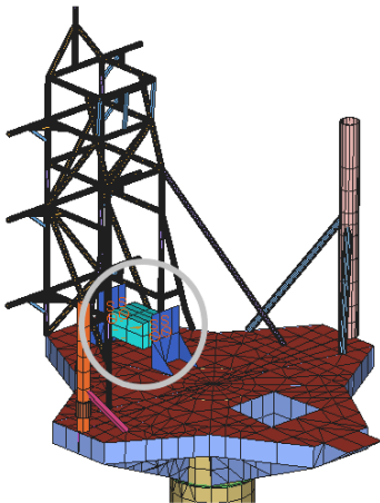
Fig. 6 FE model of dynamic vibration absorber on the radar mast platform top
