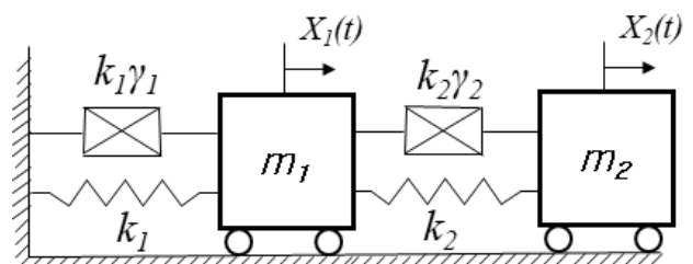
Fig. 1 Idealized 2-d.o.f system consisted of a substructure and a dynamic vibration absorber
