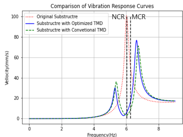
Fig. 5 Vibratory response of substructure with and without dynamic vibration absorber
