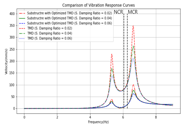
Fig. 8 Numerically evaluated vibratory response of substructure and dynamic vibration absorber according to the variation of structural damping
