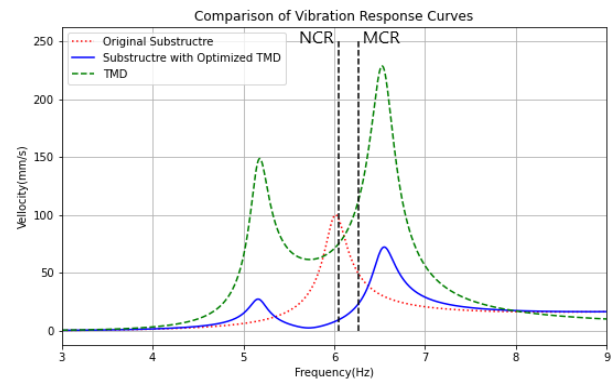
Fig. 7 Vibratory response curves obtained by FE analysis
