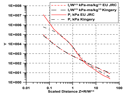
Fig. 7 Comparison of Kingery model and EU JRC model for free-air burst (Karlos, 2016)
