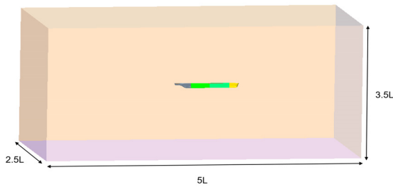
Fig. 8 Size of CFD computational domain
