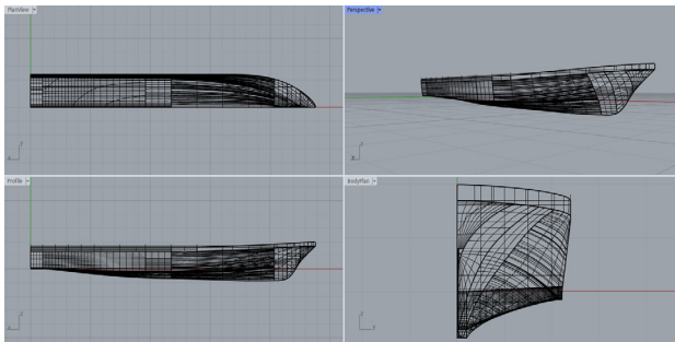
Fig. 11 The shape of a baseline hull for patrol ship
