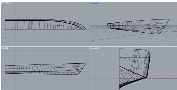
Fig. 12 The shape of a patrol ship created by Orca3D
