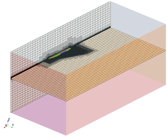
Fig. 10 Grid system
