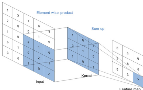
Fig. 2 An example of convolution operation
